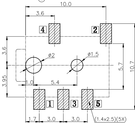
PCB HOLES(TOP VIEW) t=1.0mm NOTE: GENERAL TOLERANCE: \pm 0.05mm
