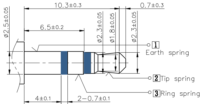
RECOMMENDED PLUG Ø2.5 3-POLE STANDARD PLUG
