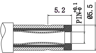
MATING PLUG
